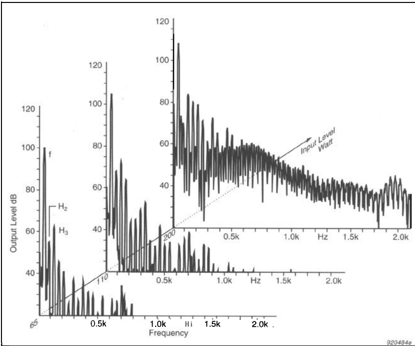
Fig. 26 Harmonic Distortion of a dynamic loudspeaker at high output levels from 110 dB SPL at 1 meter. Test signal is a 100 ms, 41 Hz tone burst. Measured in an anechoic chamber.
