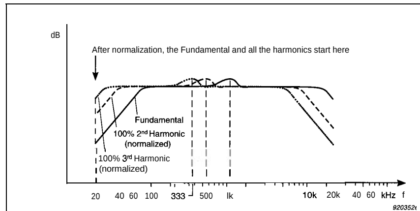
Fig. 5c Distortion Responses frequency normalized to the Fundamental Response
