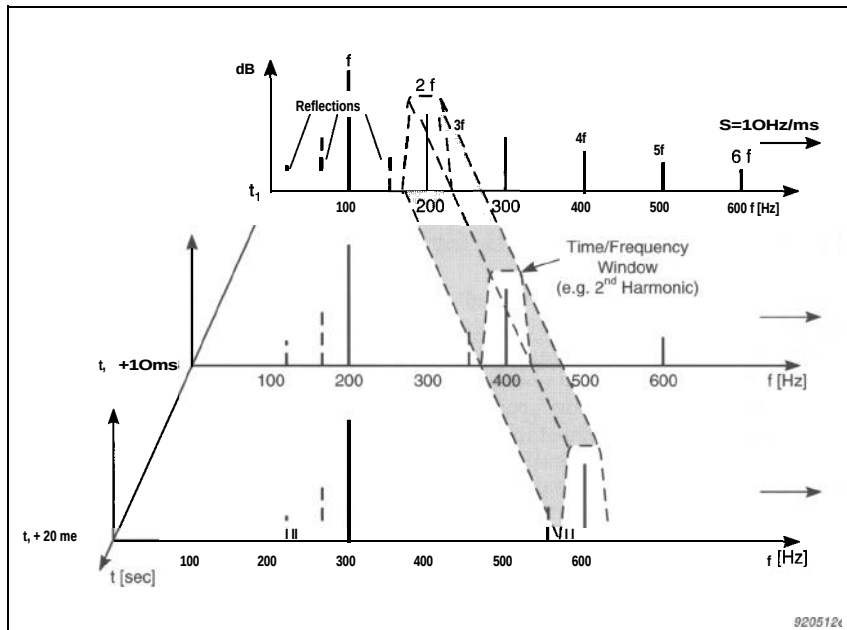
Fig. 29a Time Selective Measurements of Individual Harmonics
