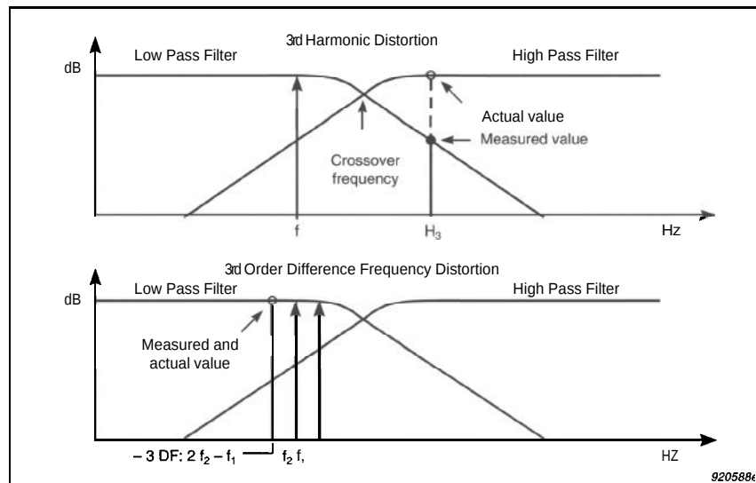
Fig. 21a Harmonic Distortion components are attenuated by filter networks while 3rd order difference frequency components remain the same level as the excitation frequencies, f_1 and f_2 (assuming 100% distortion)
