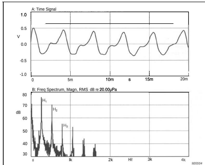
Fig. 7 Middle C (261.63 Hz) played by a Flute
