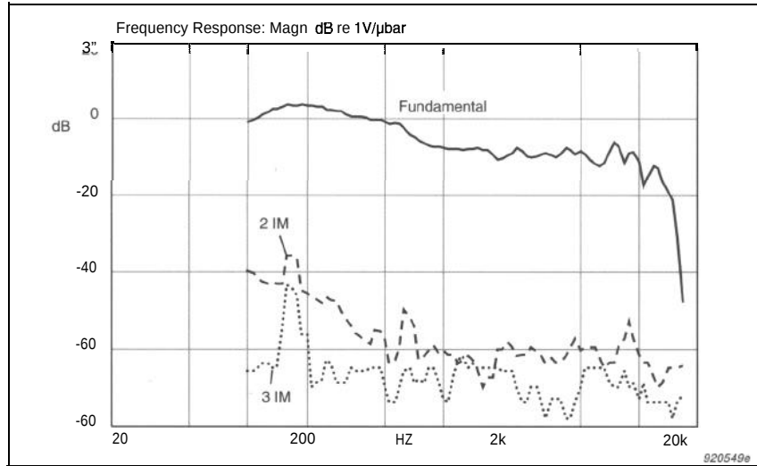
Fig. 24 IM distortion produced by an unidirectional dynamic microphone used for vocals. Input 120 dB SPL at the mouth simulator’s reference point (MRP), f_2 = 82.4 Hz, a_2 = 4a_1 (1 bar = 10^5 Pa)
