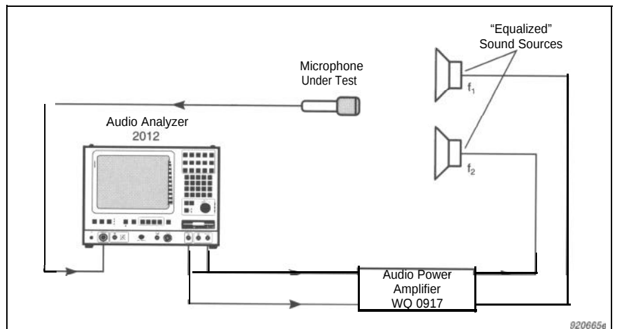
Fig. 23 Measurement setup for distortion measurements on microphones
