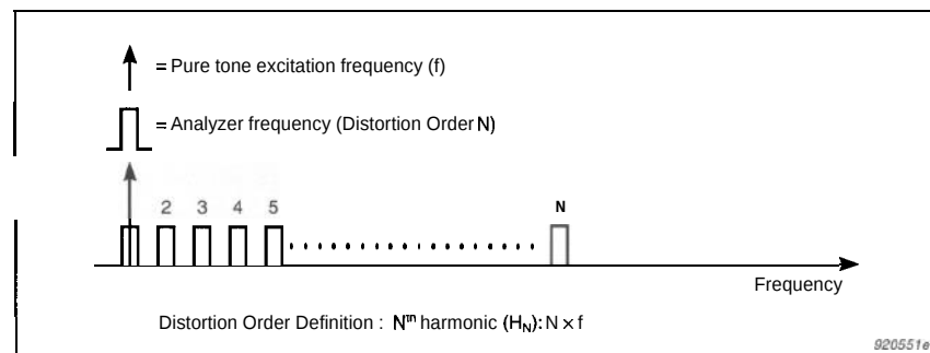
Fig. 2 Harmonic distortion
