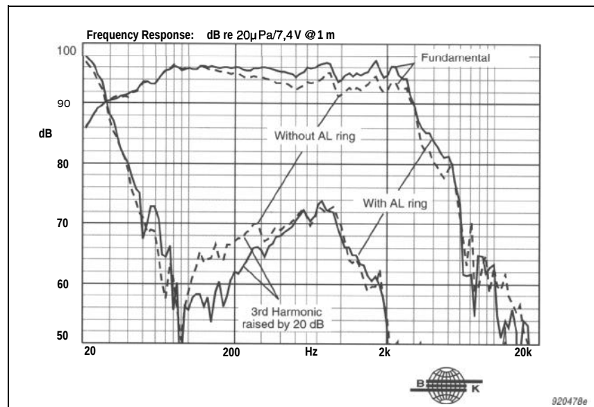
Fig. 11c 3rd Harmonic Distortion with the addition of an aluminium short-circuiting ring in the woofer's motor
