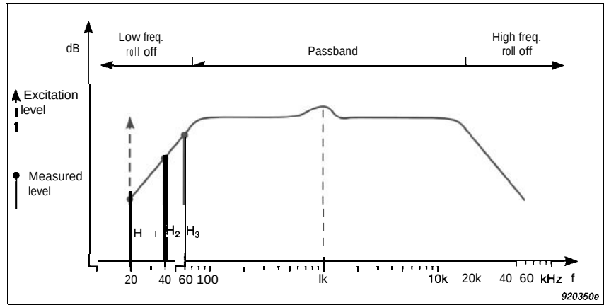
Fig. 5a Simplified representation of a transducer with a limited frequency range and a peak at 1 kHz. Fundamental response ( H_1 ), 2 nd harmonic ( H_2 ) and 3 rd harmonic ( H_3 ) of 20 Hz
