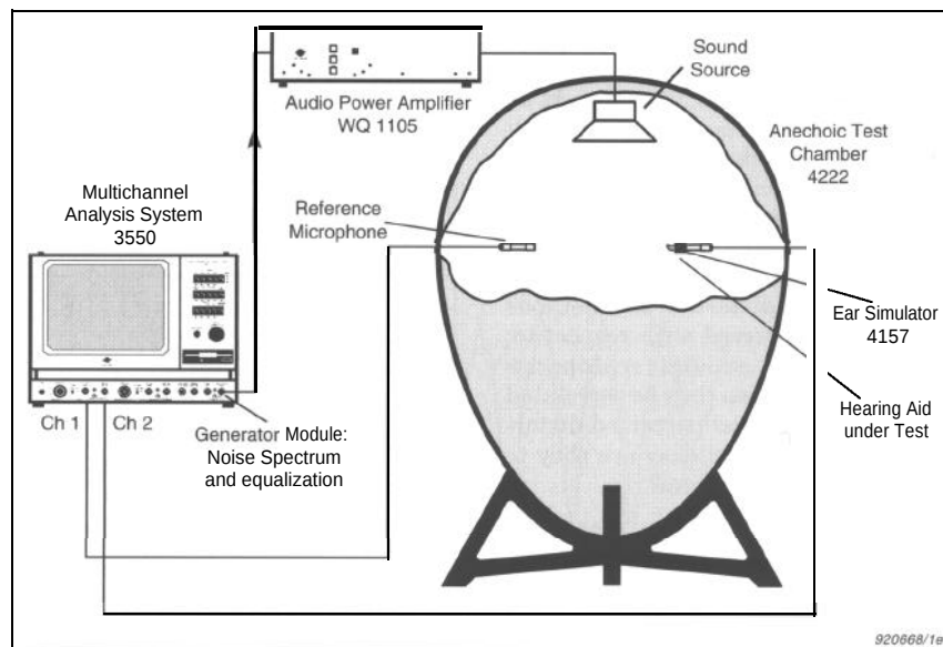
Fig. 13 Measurement setup for S-Channel measurement on Hearing Aids
