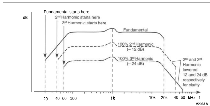
Fig. 5b Distortion Responses at the Actual Measured Frequencies (assuming 100% constant distortion vs. frequency)
