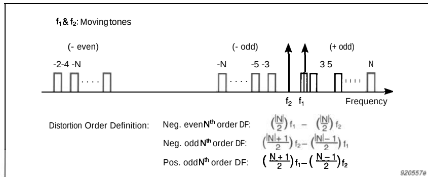
Fig. 17b DF distortion order definition
