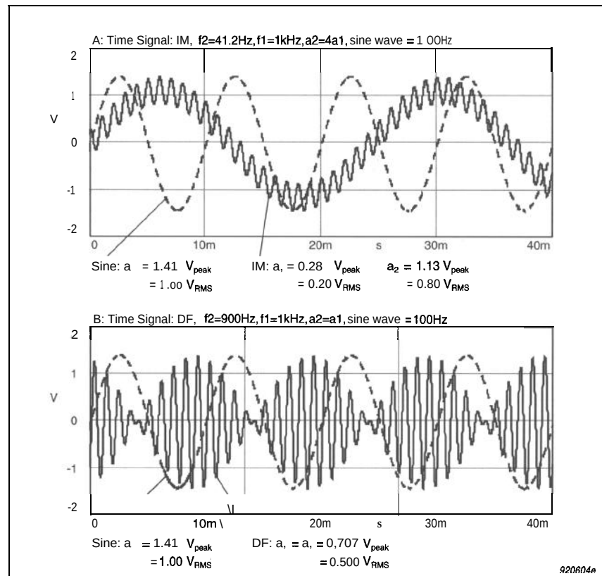
Fig. 30 The total peak value of the distortion test signal must be equal in order to compare results for different distortion test methods: a) Single sine wave (e.g. Harmonic distortion) and a Two-tone signal consisting of Two sine waves with different amplitudes (e.g. Intermodulation distortion, a_2 = 4a_1 ) b) Two-tone signal consisting of two sine waves of equal amplitude (e.g. Difference Frequency distortion, a_2 = a_1 )
