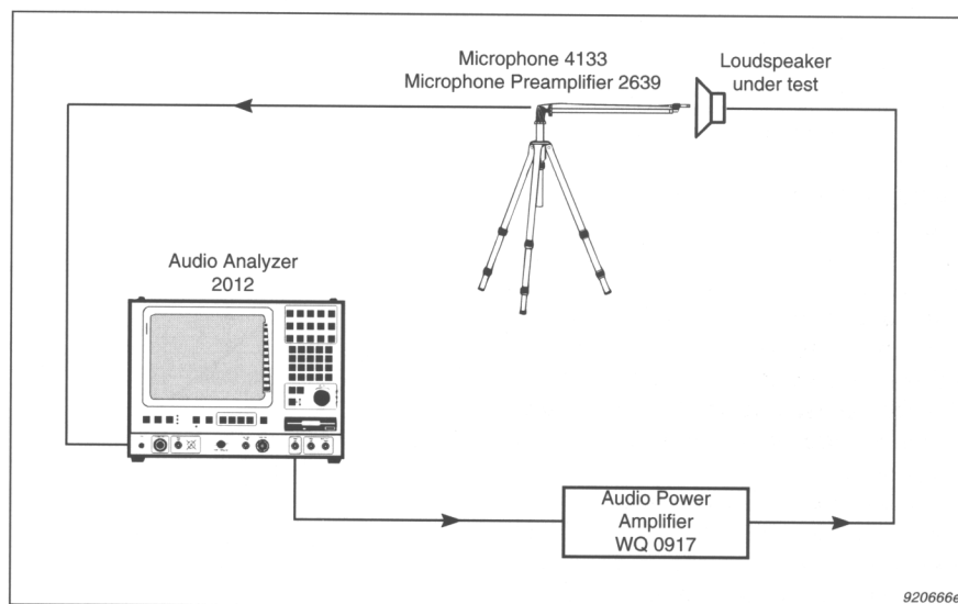
Fig. 9 Measurement setup for Rub and Buzz measurement on a loudspeaker
