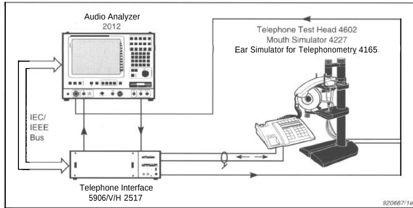
Fig. 19 Measurement setup for measurement on telephones
