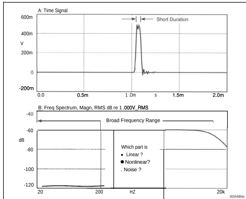
Fig. 12 A Pulse and its Frequency Spectrum
